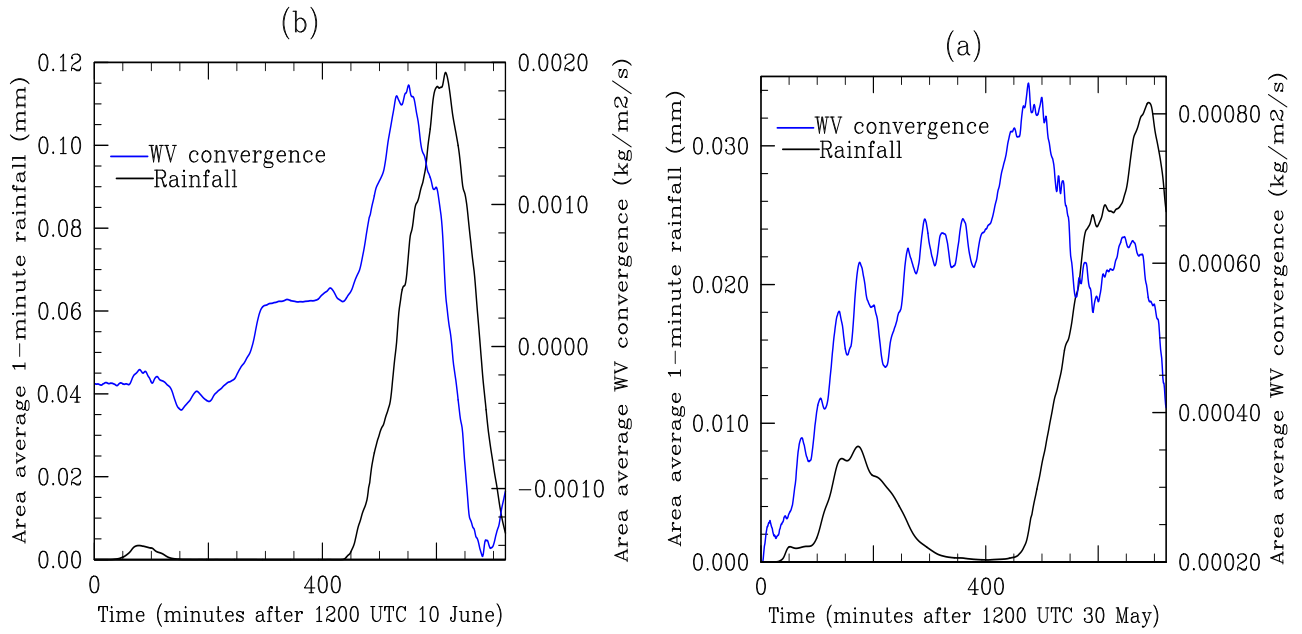
Figure 7: Timeseries of 1-minute rainfall accumulation (mm, black) and low-level water vapor convergence ( \text{kgm}^{-2}\text{s}^{-1} , blue) averaged over a 151km square box for (a) case 2 and (b) case 3.
