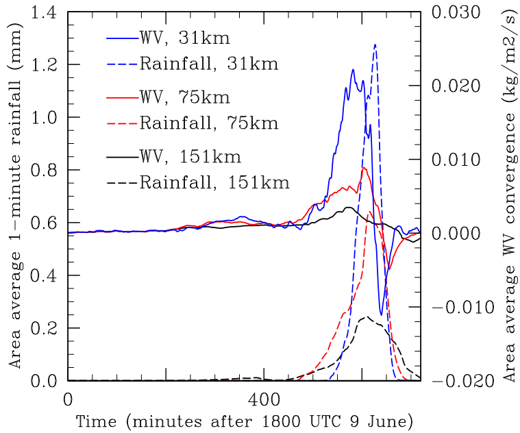
Figure 5: Timeseries of 1-minute rainfall accumulation (mm, dashed) and low-level water vapor convergence ( \text{kgm}^{-2}\text{s}^{-1} , solid) averaged over square boxes of length 151km (black), 75km (red) and 31km (blue).
