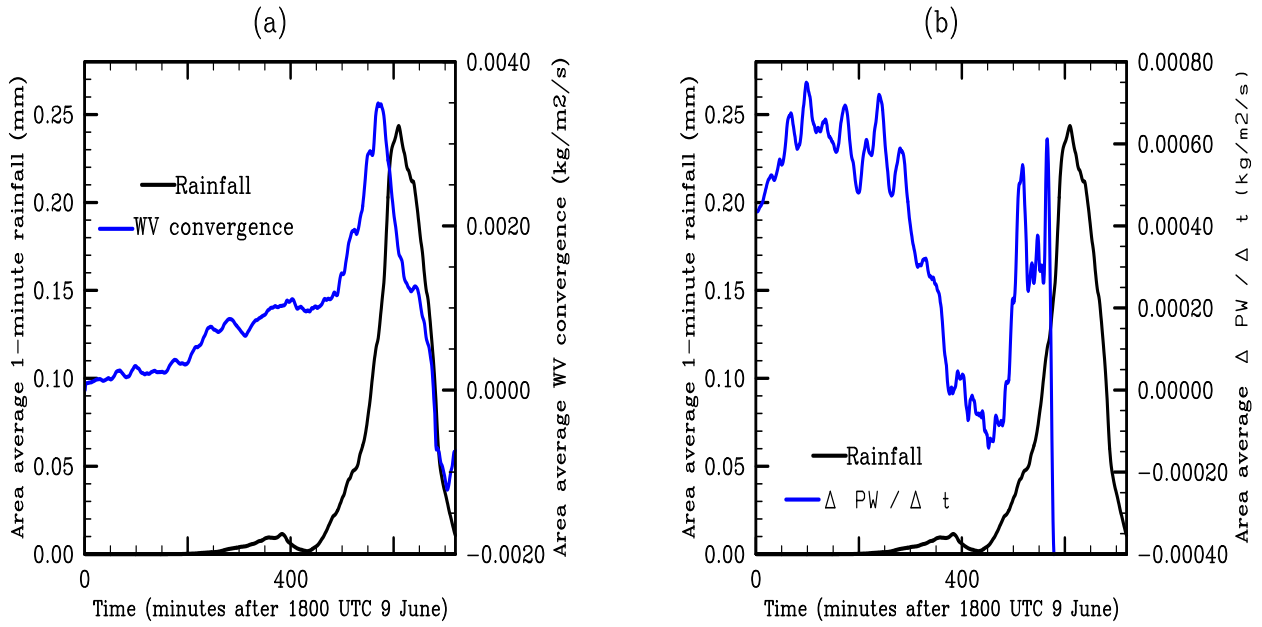
Figure 3: (a) Timeseries of 1-minute rainfall accumulation (mm, black) and low-level water vapor convergence ( \text{kgm}^{-2}\text{s}^{-1} , blue), and (b) Timeseries of 1-minute rainfall accumulation (mm, black) and time rate of change of PW using \Delta t = 1\text{min} ( \text{kgm}^{-2}\text{s}^{-1} , blue). All quantities are area averages taken over the sub-region shown in Fig. 1.
