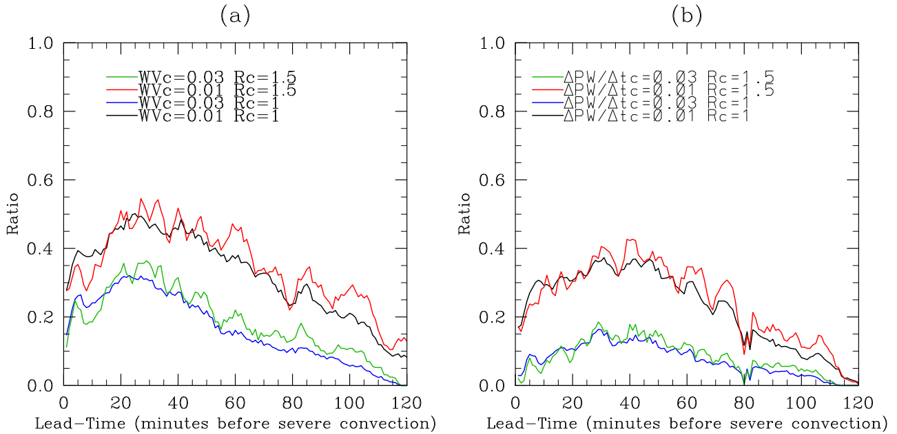
Figure 4: Ratio of the number of grid points exceeding a rainfall threshold to the number of those grid point exceeding (a) a water vapor convergence threshold and (b) a \Delta PW / \Delta t threshold, for different thresholds.
