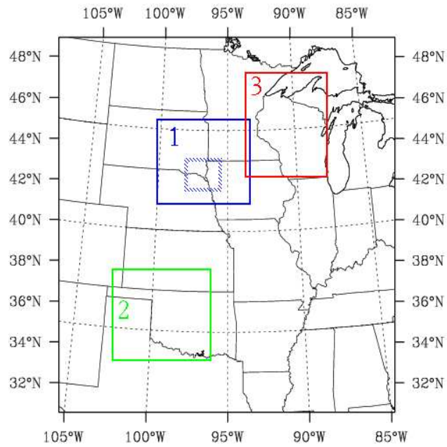
Figure 1: The parent domain (black) and nested domains for case 1 (blue), case 2 (green) and case 3 (red). Outlined in a blue dashed line is a sub-region of the nested domain for case 1 used to calculate area average quantities.
