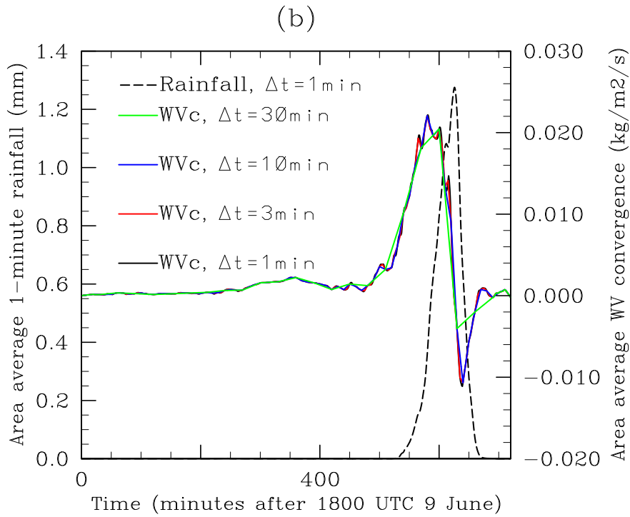
Figure 6: Timeseries of 1-minute rainfall accumulation ( \text{mm} , dashed) and low-level water vapor convergence ( \text{kgm}^{-2}\text{s}^{-1} , solid) averaged over a 31\text{km} square box using (a) data of degraded spatial resolution and (b) data of degraded temporal resolution.
