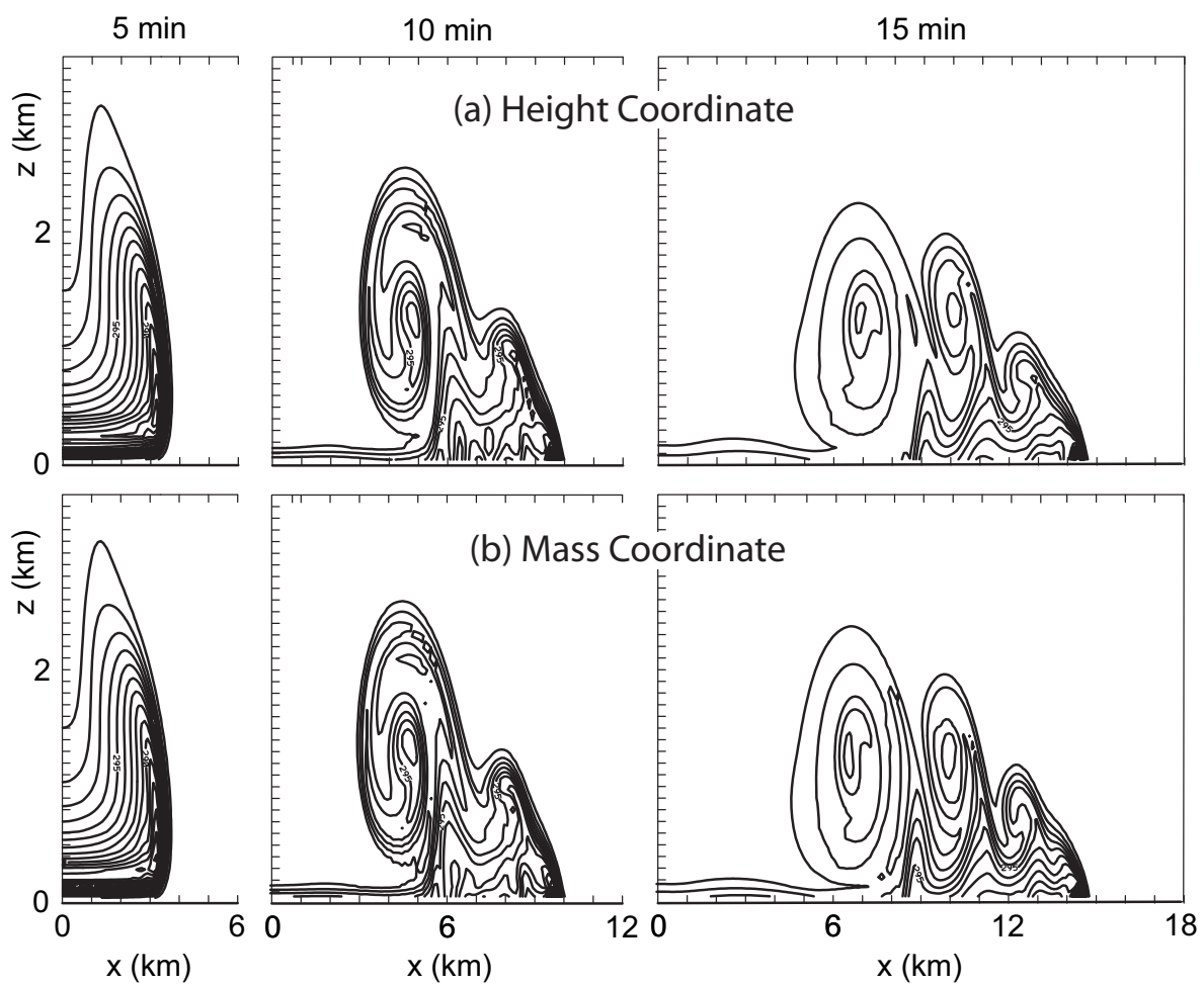
FIGURE 1. Potential temperature field for Straka et al. (1993) 2-D density-current benchmark case for (a) height coordinate and (b) mass coordinate simulations for \Delta x = \Delta z \simeq 100 \text{ m} . Contour interval is 1 K.
