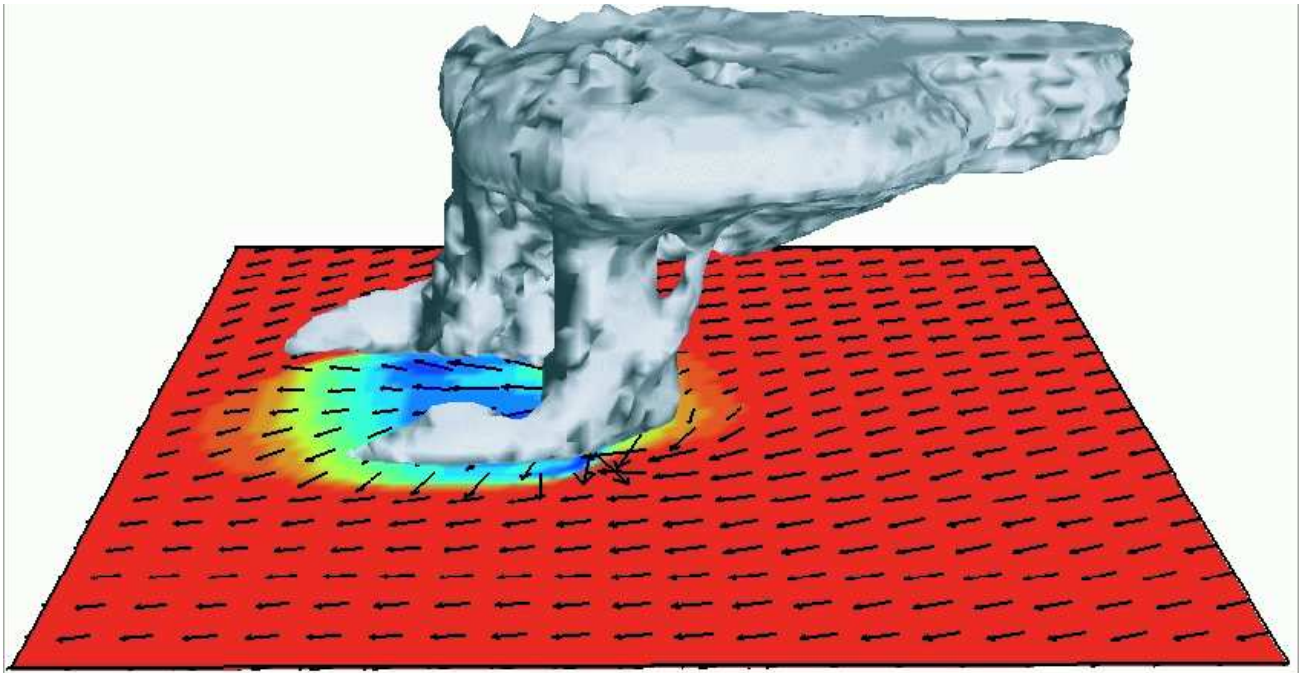
FIGURE 2. Simulated splitting supercell thunderstorms evolving in strong environmental wind shear, displayed at 2 h. The cloud field is shaded in gray, surface temperature is colored in shades ranging from red (warm) to blue (cold), and surface wind vectors are included at every fourth interval. The model integration employed \Delta x = \Delta y = 1 km, \Delta z \simeq 500 m, within an 80 \times 80 \times 20 km domain. (from Klemp and Skamarock 2004)
