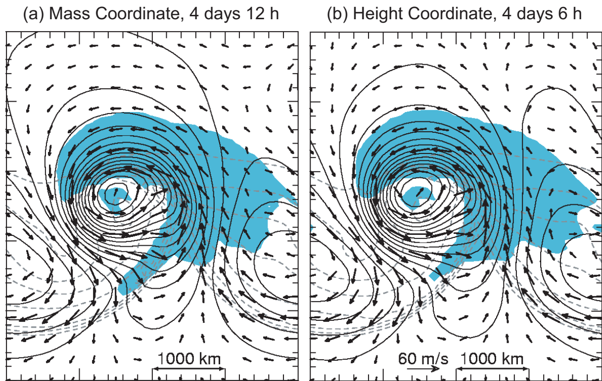
FIGURE 3. Baroclinic wave in a channel for the (a) mass coordinate and (b) height coordinate simulations, depicting the surface pressure (solid lines, c.i. = 4 mb), temperature (dashed lines, c.i. = 4 K), and cloud field (shaded in blue). The model grid is \Delta x = \Delta y = 100 km and \Delta z \approx 250 m within a 4000 \times 6000 \times 9 km domain.
