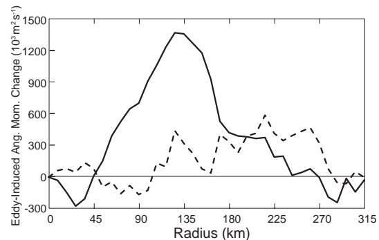
Figure 4. Radial profiles eddy-induced angular momentum changes from CTRL (heavy solid) and BMJ1 (dashed). All quantities represent averages from 21 h to 36 h and from roughly 0 to 2 km MSL. All quantities represent averages between simulation hours 21 and 36 and over the lowest 2 km of the model domain.
