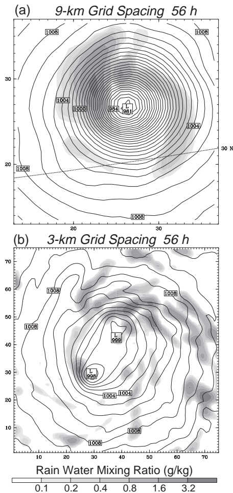
Figure 6. Comparison of sea-level pressure and rain water mixing ratio at lowest model level at 56 h (2000 UTC 9 September) for (a) CTRL and (b) 4D21.
