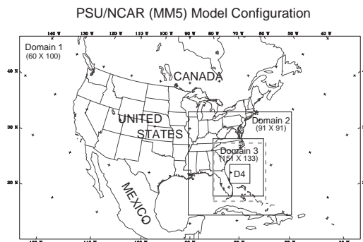
Figure 1. Domain configuration, including stationary location of Domain 4 (3 km grid spacing, 151 \times 151 points). The dashed gray box defines the domain of the single domain simulation with 1.2-km grid spacing.
