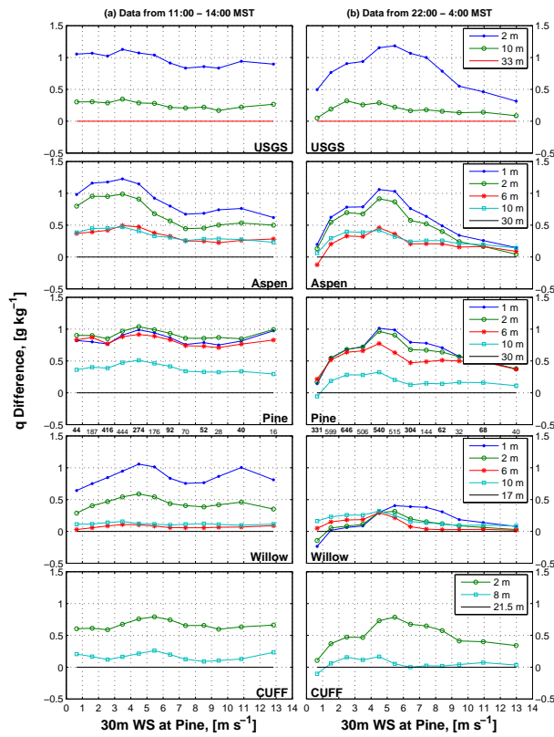
Figure 3: As in Fig. 2, but for specific humidity q .
