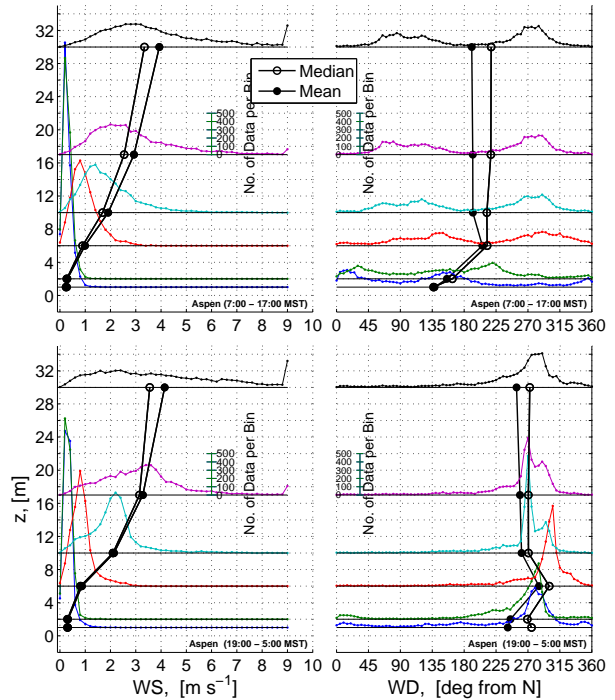
Figure 11: Frequency distributions of (a) wind speed WS, and (b) wind direction WD at different levels on the Aspen tower for daytime (top panels) and nighttime (lower panels).
