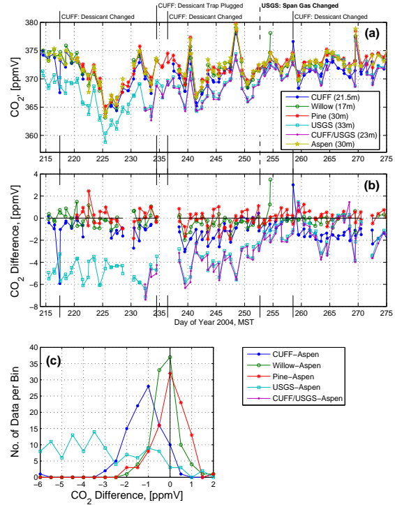
Figure 9: Time series of (a) \text{CO}_2 measured between 11:00-14:00 MST from 1 August to 30 September, 2004, (b) the difference in \text{CO}_2 between the highest level on each tower (the 30-m \text{CO}_2 at Aspen is used as the reference), and (c) the frequency distribution of the difference between the \text{CO}_2 measurements. The \text{CO}_2 values are 2-hour medians. The vertical lines (and corresponding text) in the top panel specify any changes to the measuring systems.
