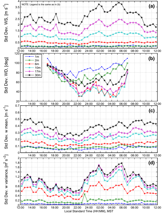
Figure 15: As in Figure 13, except the standard deviation of the data within each bin are shown.
