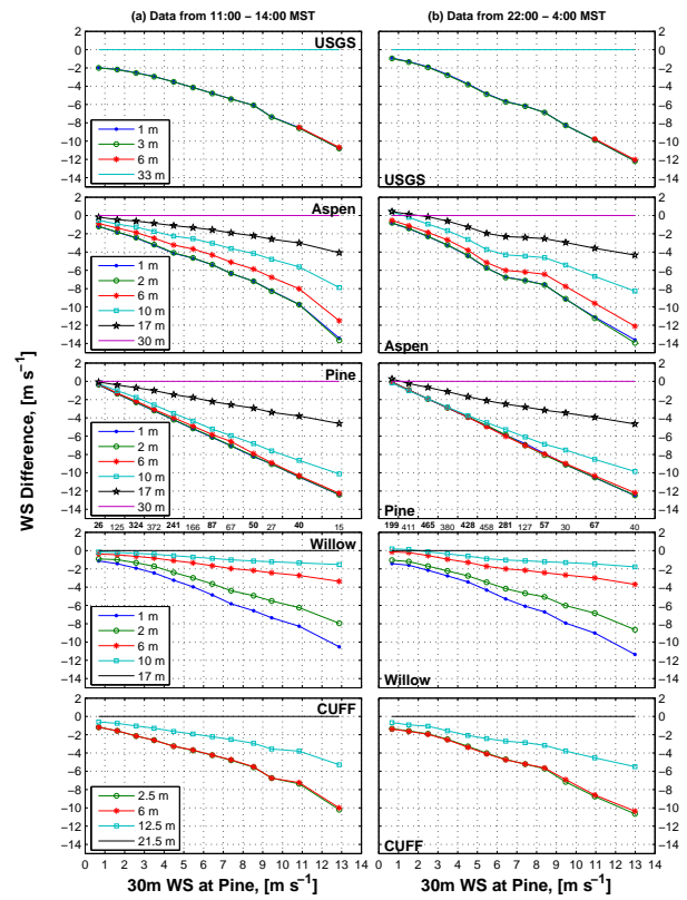
Figure 5: As in Fig. 2, but for wind speed WS.
