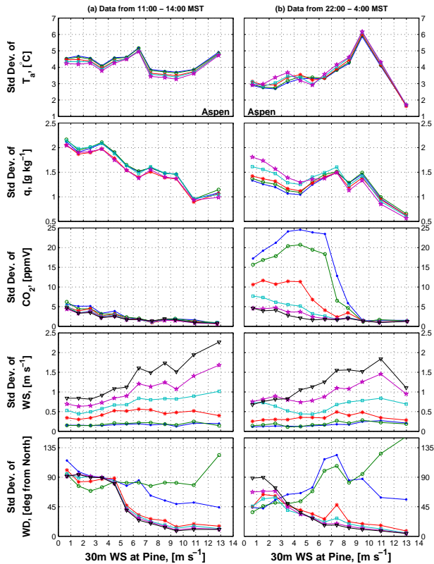
Figure 10: The standard deviation of the data shown in Fig. 7. The legend for each panel is the same as that shown in Figs. 7 and 8.
