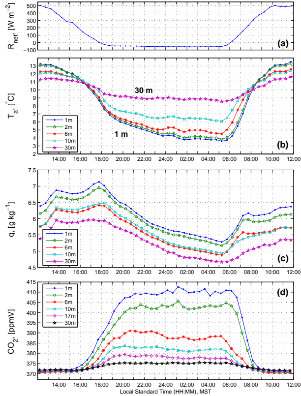
Figure 12: Half-hourly binned mean measurements from August and September, 2004 at the Aspen Tower for (a) net radiation R_{net} , (b) air temperature T_a , (c) specific humidity q , and (d) carbon dioxide CO_2 . Five-minute mean data are used for R_{net} , T_a , and q while 15-minute data are used for CO_2 .
