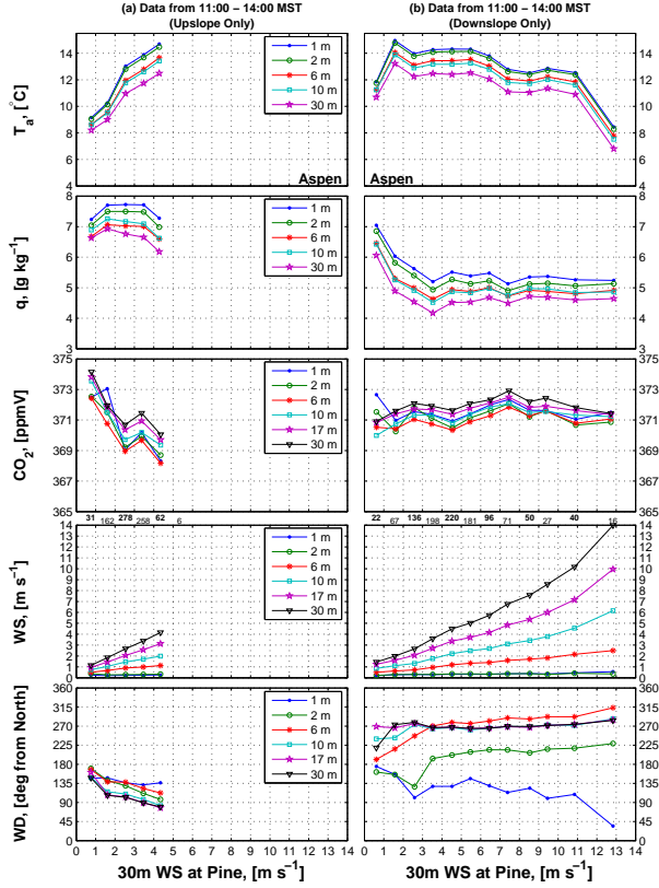
Figure 8: Daytime data from Fig. 7 (column a), but separated into (a) upslope and (b) downslope conditions at 30 m.
