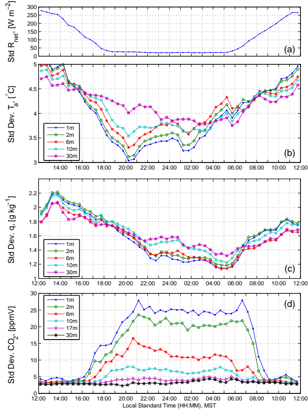
Figure 14: As in Figure 12, except the standard deviation of the data within each bin are shown.
