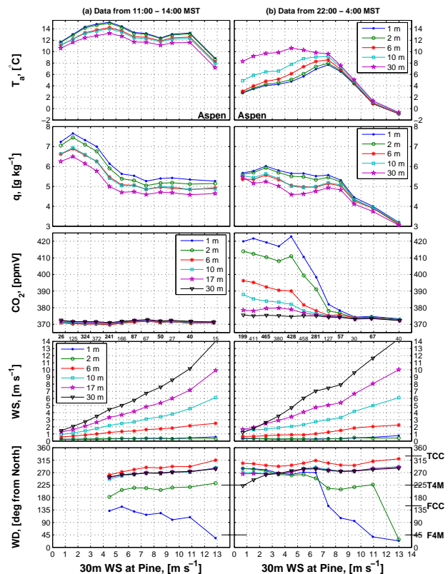
Figure 7: Aspen tower mean air temperature T_a , specific humidity q , carbon dioxide \text{CO}_2 , wind speed WS, and wind direction WD binned by the 30-m WS measured at the Pine tower. The horizontal lines and text in the WD panels indicate the direction for air flowing toward (TCC) or from (FCC) Como creek and, for air flowing toward (T4M) or from (F4M) the Fourmile creek drainages (these directions are relative to the Aspen tower).
