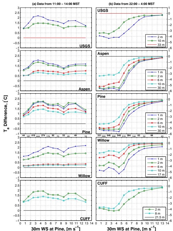
Figure 2: The vertical gradient of air temperature T_a measured at each tower binned by the 30m-WS at the Pine tower (the lower levels are subtracted from the highest measurement level). Note that the y-axis range of the left and right panels differ. The number of 5-min data values for each bin is shown between the panels for Willow and Pine (the number of possible 5-min samples is 2196 for the daytime data and 4392 for the nighttime).
