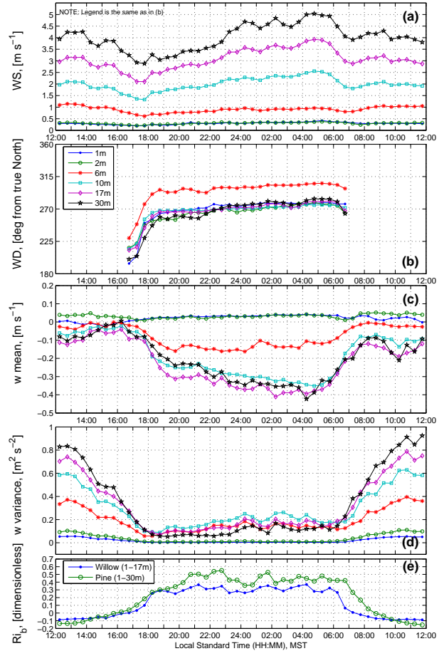
Figure 13: Half-hourly binned mean measurements at the Aspen Tower for (a) wind speed WS , (b) wind direction WD , (c) 5-min vertical wind (mean), (d) 5-min vertical wind variance, and (e) bulk Richardson number.
