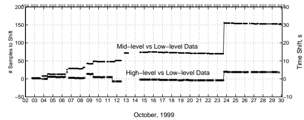
Figure 5: Time-stamp differences based on the 22.1 m thermocouple temperature data. Differences are relative to the low-level data logger for the entire experiment. Values are calculated based on 3-hour time periods (see text for details).
