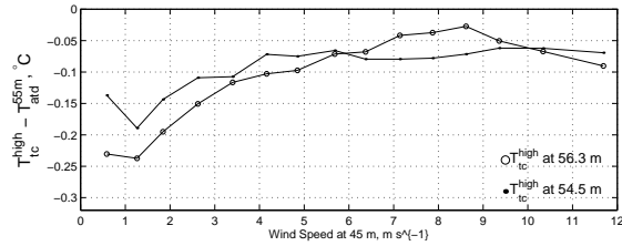
Figure 4: The difference between the thermocouple and aspirated temperature measurements versus wind speed. Only data between 18:00 and 6:00 CDT are considered.
