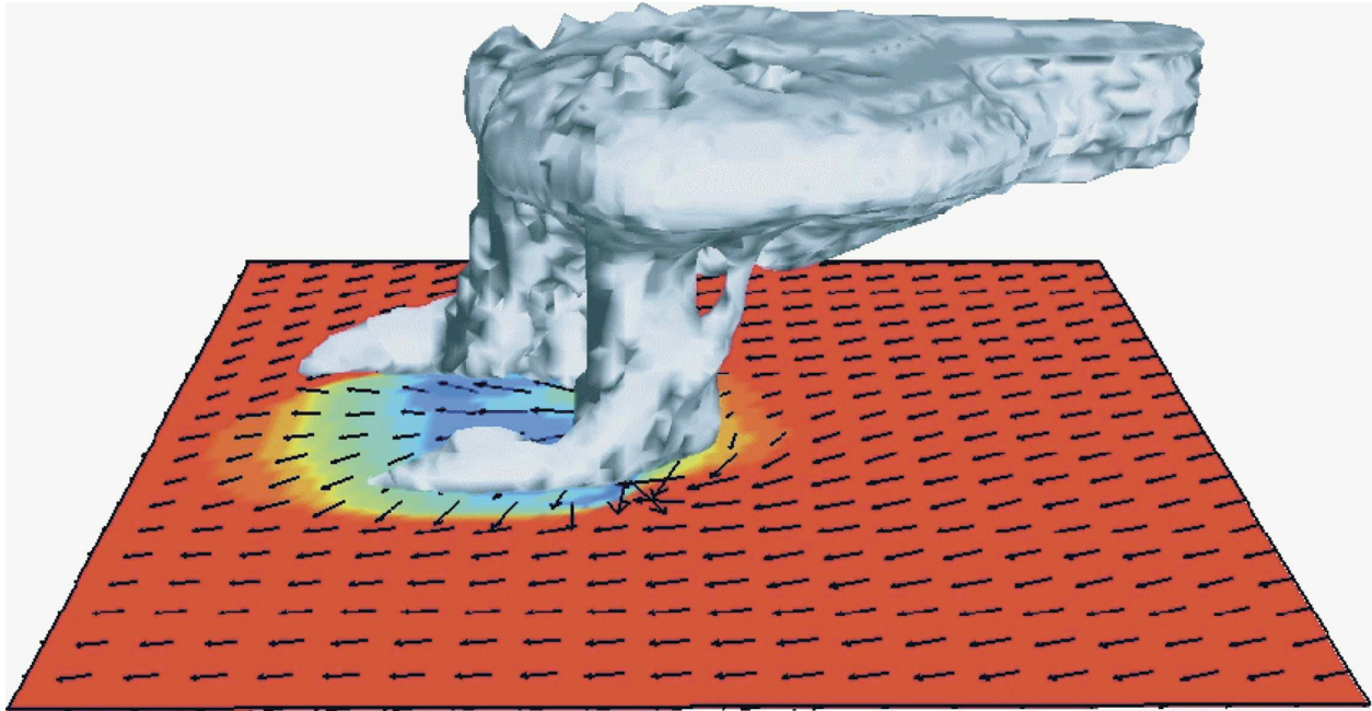
FIG. 2. Simulated splitting supercell thunderstorms evolving in strong environmental wind shear, displayed at 2 h. The cloud field is shaded in gray, surface temperature is colored in shades ranging from red (warm) to blue (cold), and surface wind vectors are included at every fourth interval. The model integration employed \Delta x = \Delta y = 1 km, \Delta z = 500 m, within an 80 \times 80 \times 20 km domain (from Klemp and Skamarock 2004).
