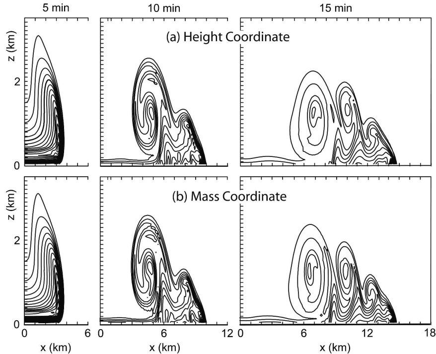
FIG. 1. Potential temperature field for Straka et al. (1993) 2D density-current benchmark case for (a) height-coordinate and (b) mass-coordinate simulations for \Delta x = \Delta z \approx 100 m. Contour interval (CI) is 1 K.
