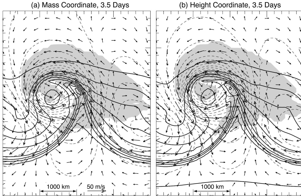
FIG. 3. Baroclinic wave in a channel for the (a) mass-coordinate and (b) height-coordinate simulations at 3.5 days, depicting the temperature (solid lines, CI = 4 K), cloud field (shaded), and horizontal wind vectors at z = 150 , together with surface pressure (dashed lines, CI = 4 mb). The model grid is \Delta x = \Delta y = 100 km and \Delta z \approx 250 m within a 4000 \times 6000 \times 16 km domain.
